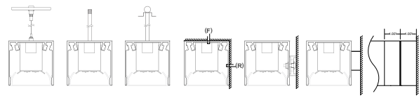
(S) Aircraft Cable (P) Rigid Stem (PV) Swivel Stem (F) Ceiling Mount (M) Mullion Blocks (H) Horizontal Setoff Bracket (J) Span (R) Direct Wall Mount (JS) Partial Span
